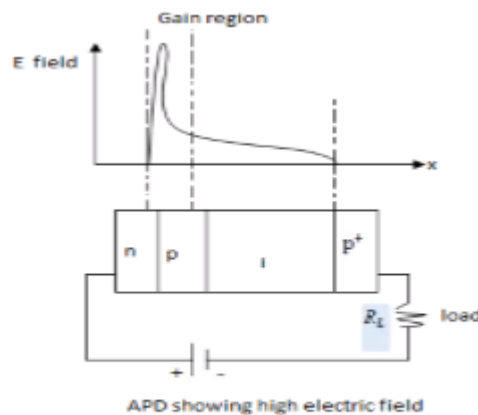
Figure 3.12: APD
