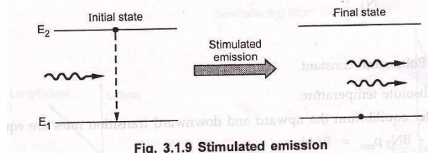
Fig. 3.1.9 Stimulated emission
