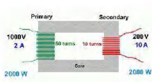
Figure 3.2.3: Step-Down Transformer
